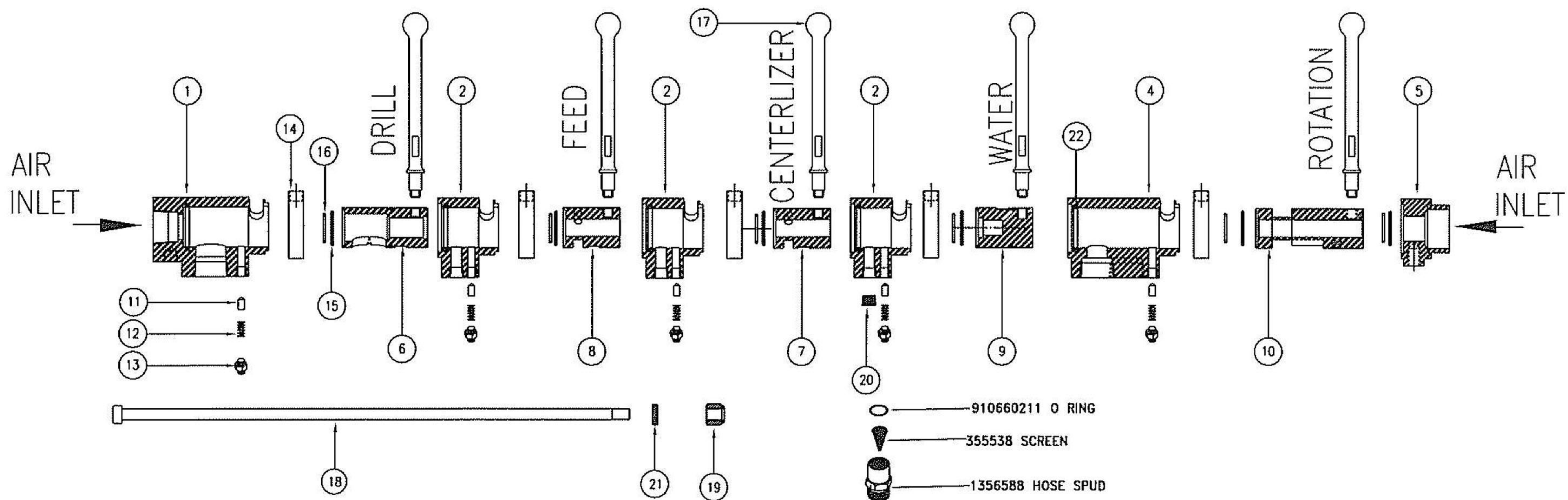
JC45 FILTER ASSEMBLY
